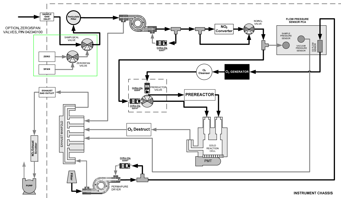
Figure 3-1: Pneumatic Diagram With Zero/Span Option
